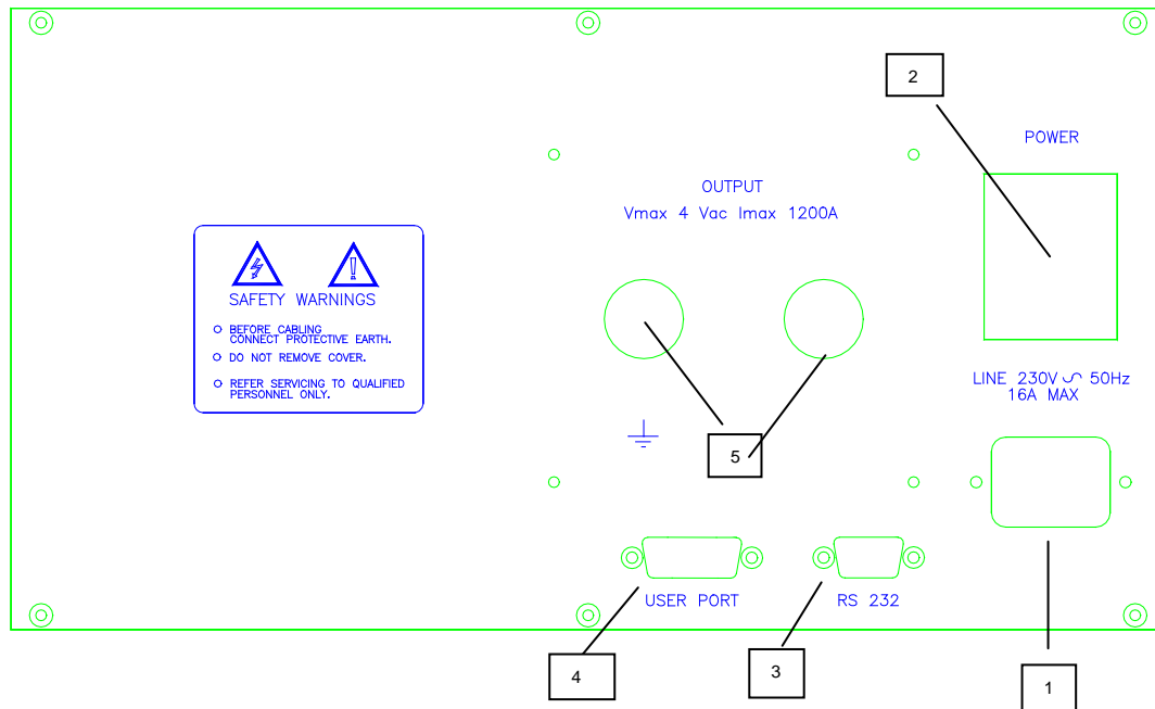
Fig. 1-3 Rear Panel
