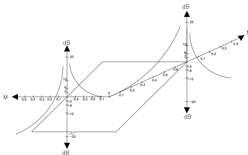
Fig. 4-1: Characteristics of the field generated by a square induction coil (1m side) in its plane
